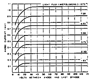
TENTATIVE AVERAGE ANODE CHARACTERISTIC
