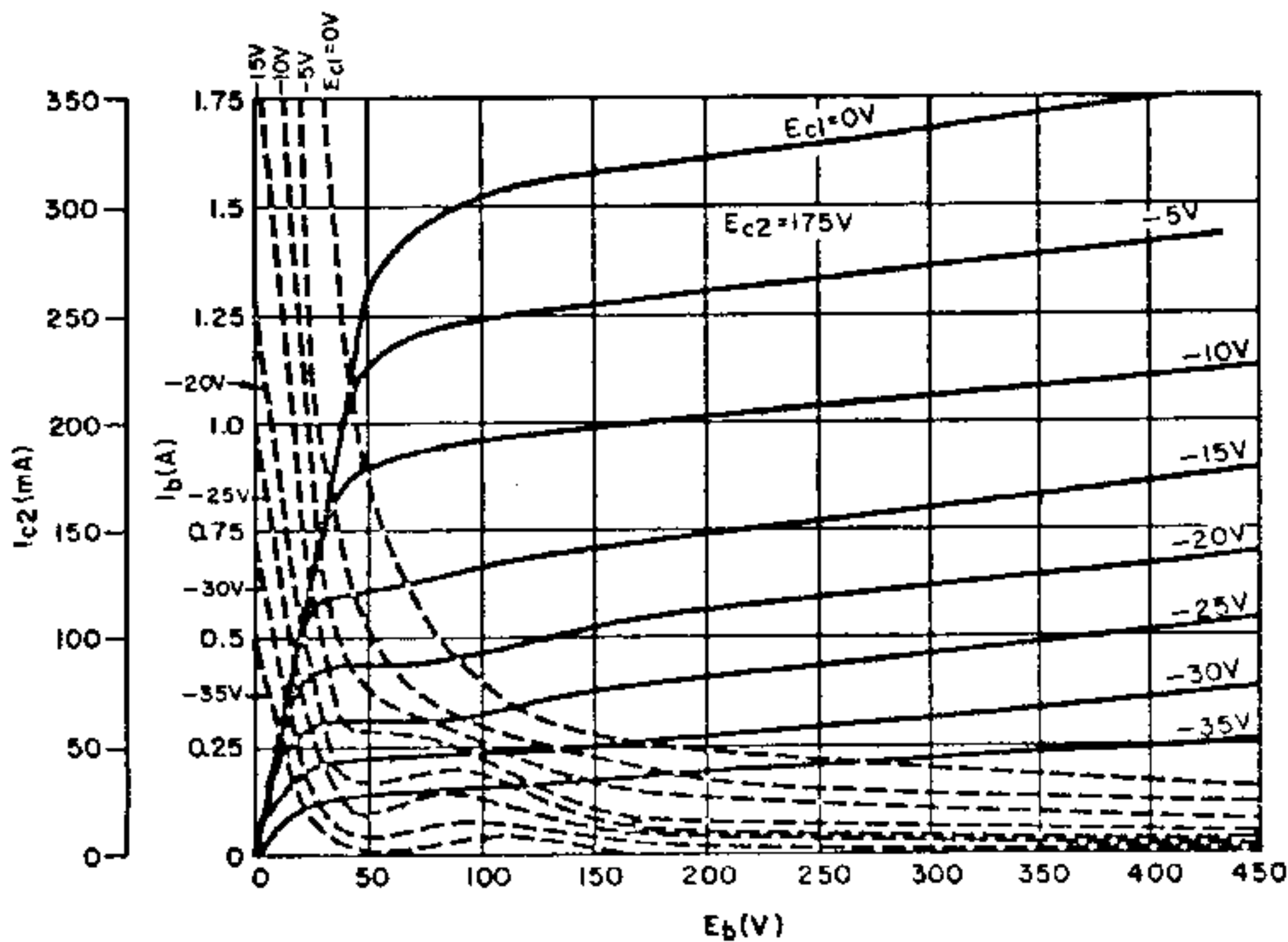
Plate Characteristics
